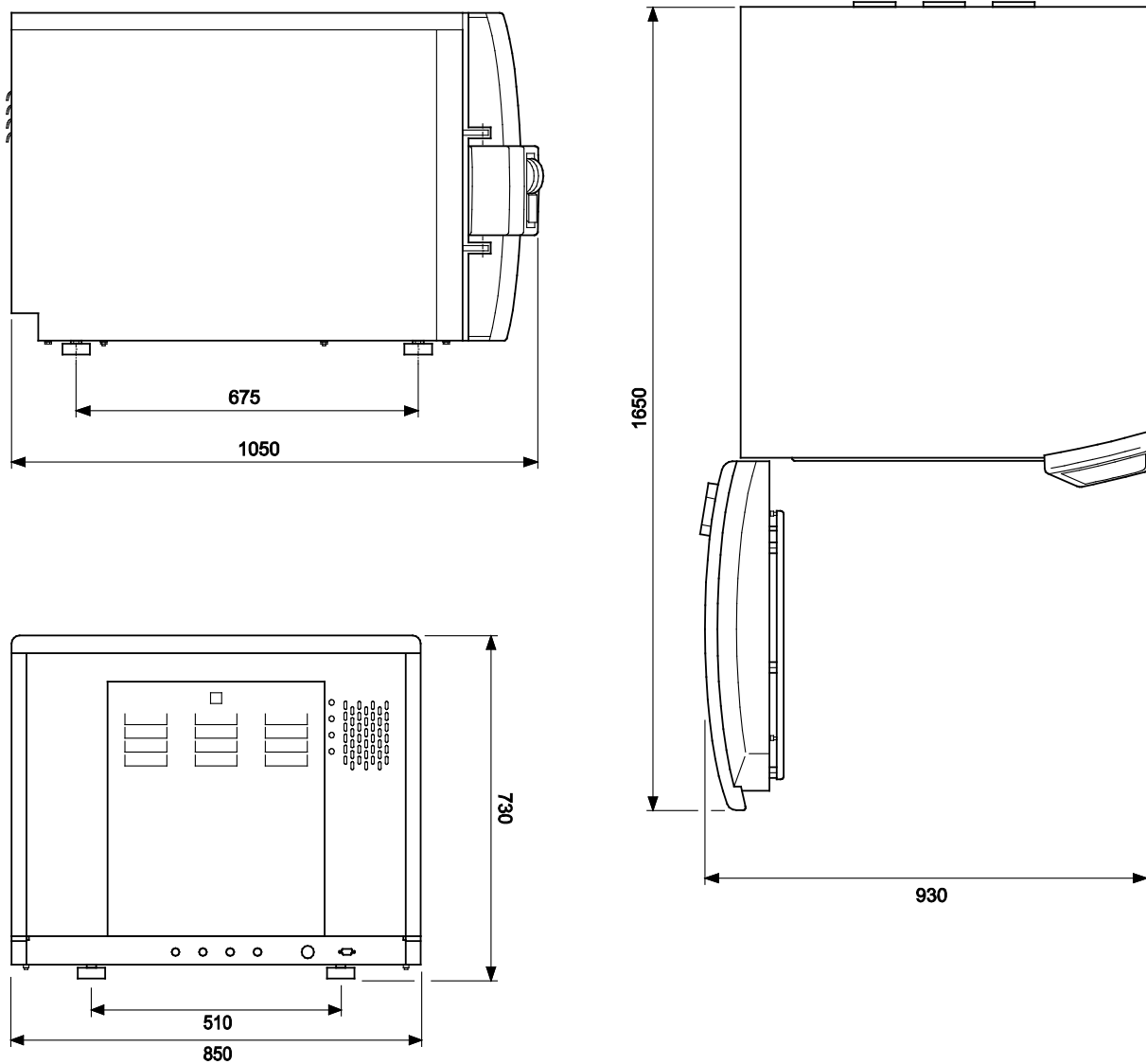
Fig. 6: Outer dimensions of Systec DX/DE-150
