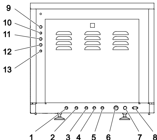
Fig. 7: Systec DX/DE-45 with automatic demineralised water supply option, back view
