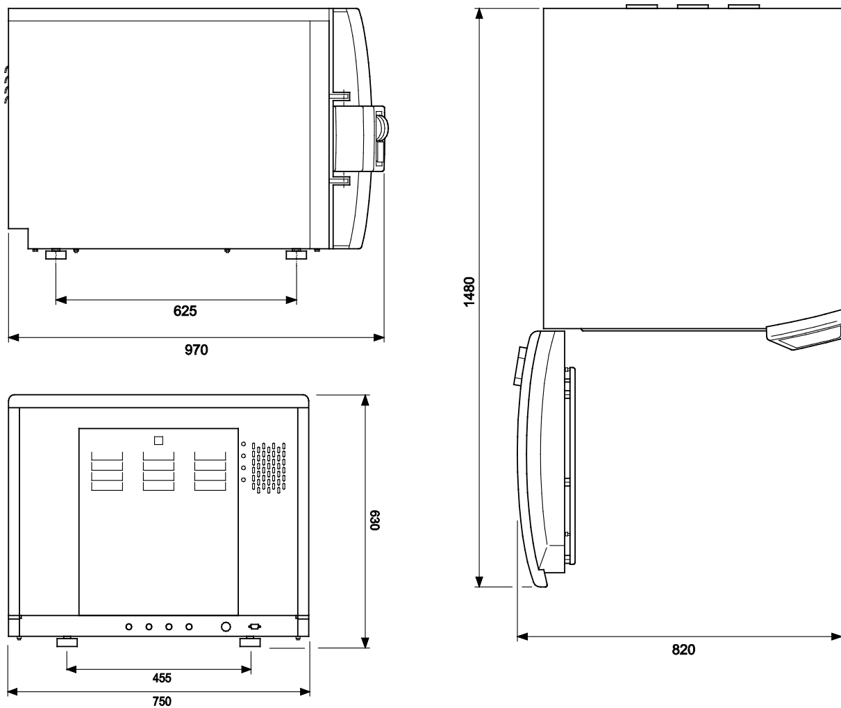
Fig. 4: Outer dimensions of Systec DX/DE-90
