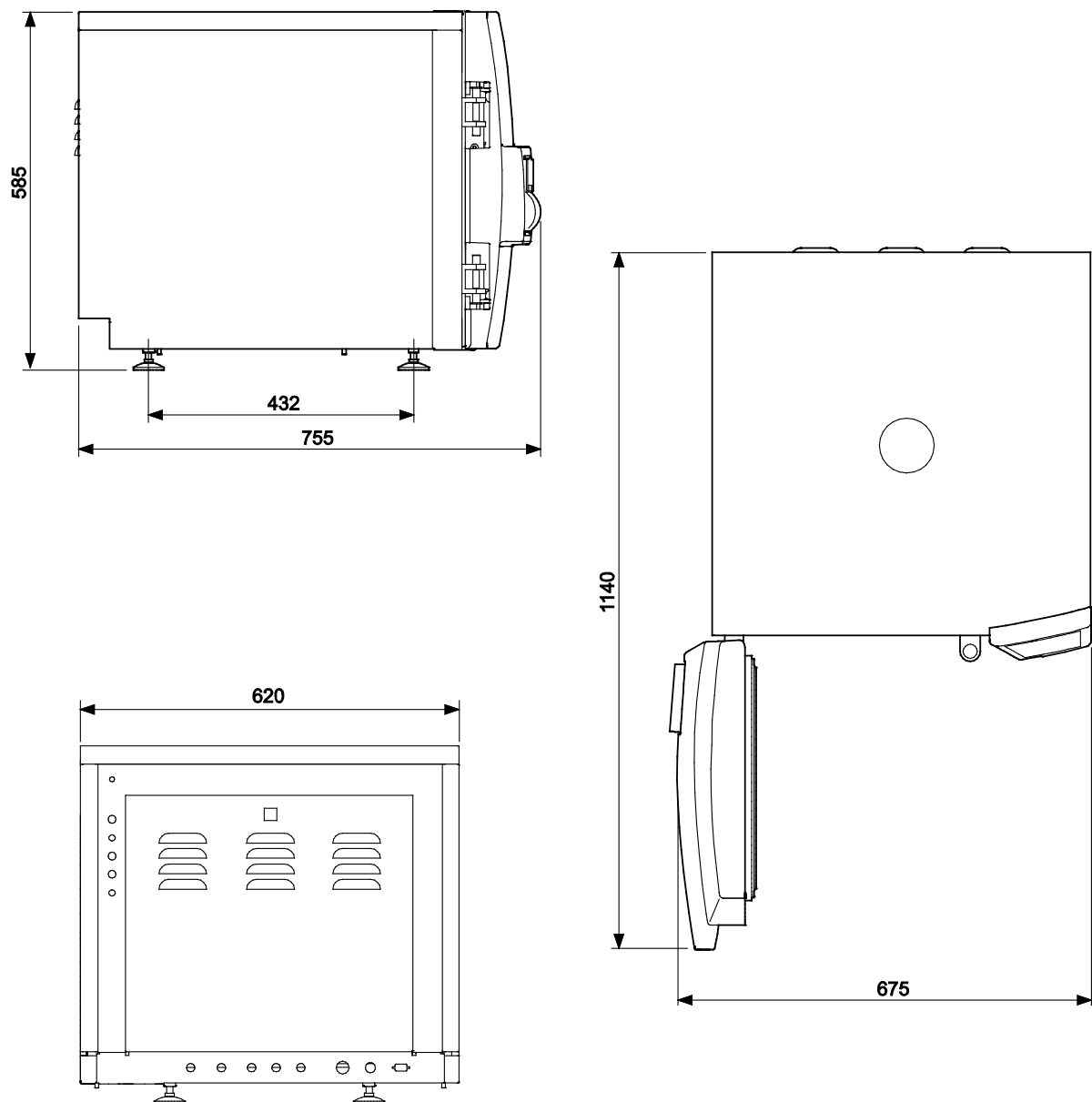
Fig. 2: Outer dimensions of Systec DX/DE-45
