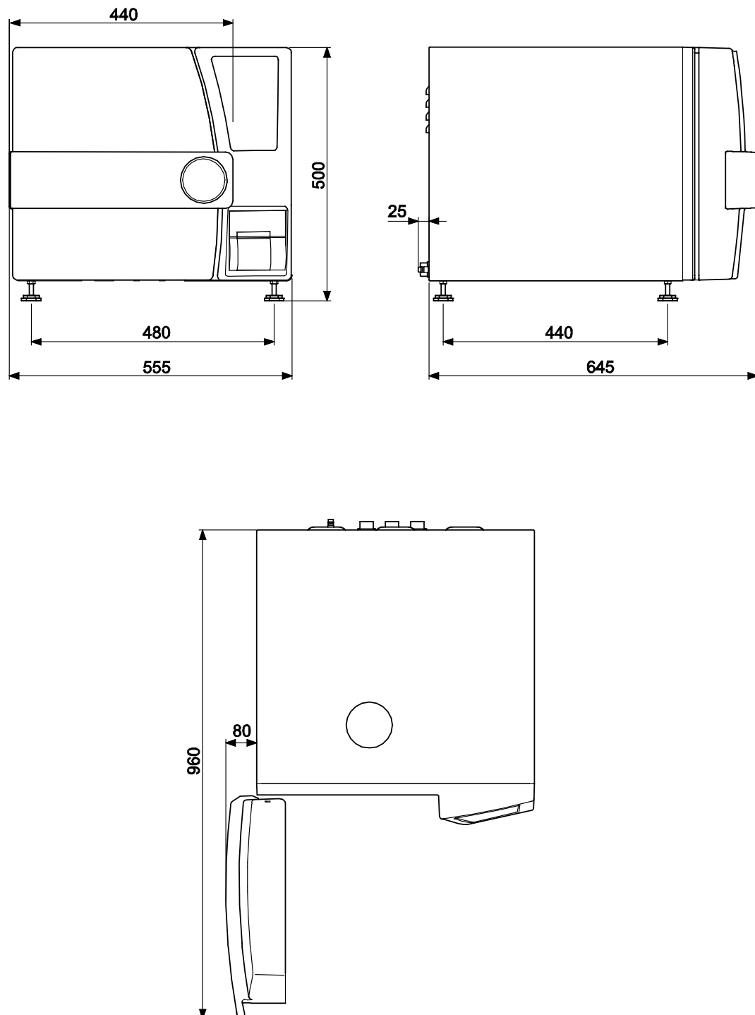
Fig. 1: Outer dimensions of Systec DX/DE-23
