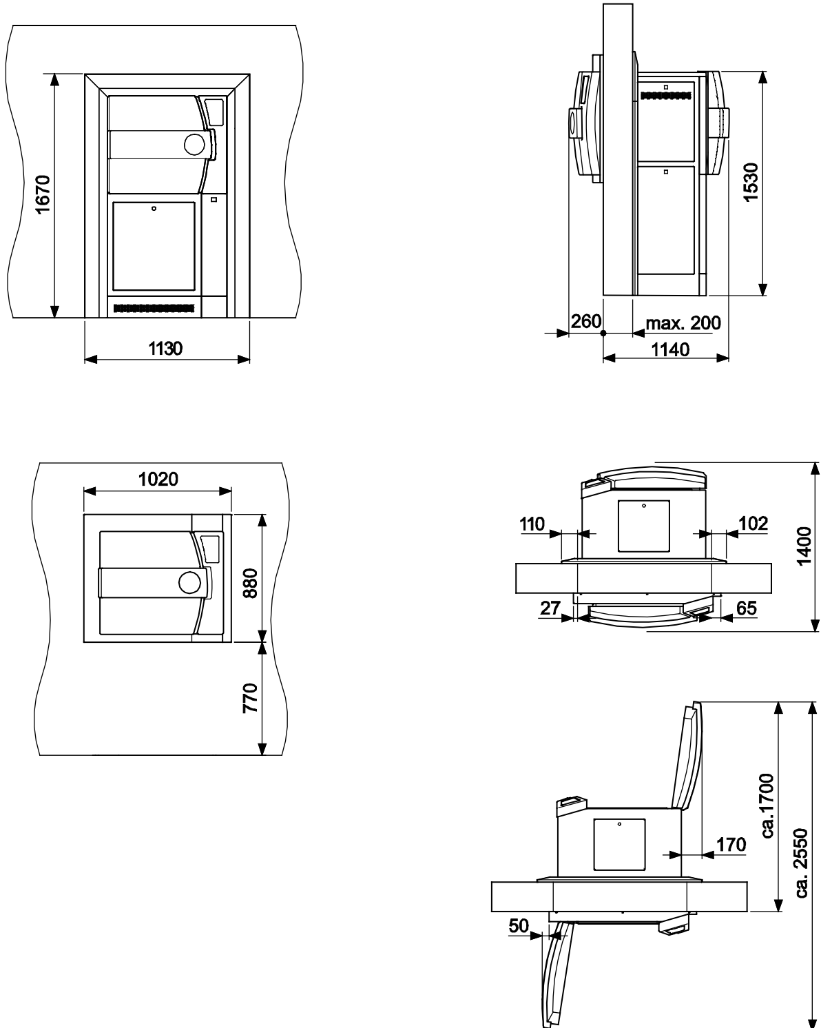
Fig. 10: Outer dimensions of Systec DX-200 2D
