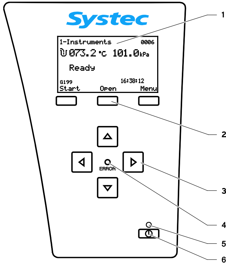
Fig. 10: Systec DX/DE Series; controller
