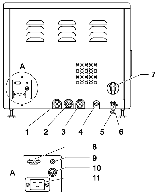
Fig. 6: Systec DE-23 with automatic demineralised water supply option, back view
