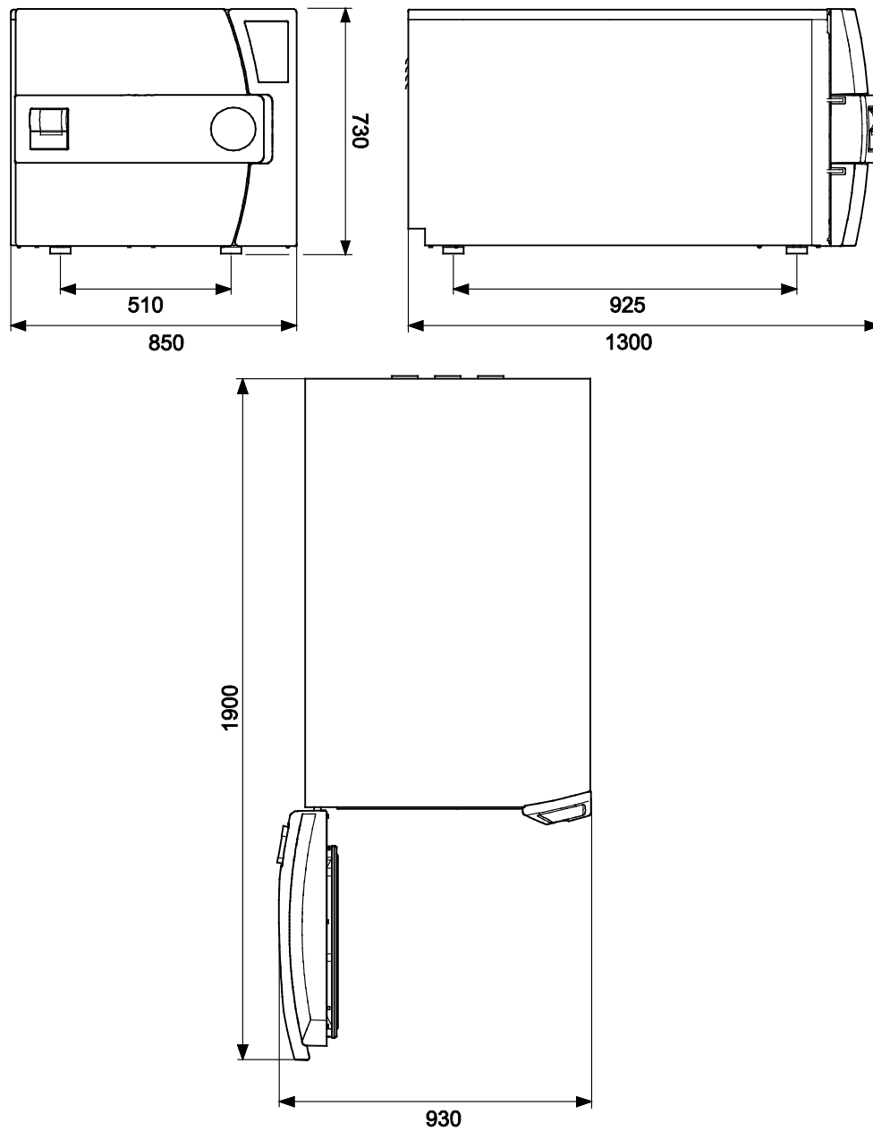
Fig. 7: Outer dimensions of Systemec DX/DE-200
