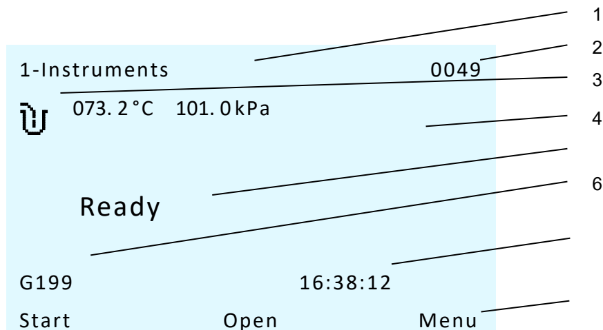
Fig. 3: Control unit display with appliance on standby (door closed)
