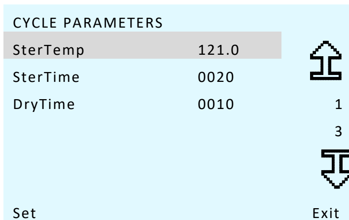
Fig. 30: Adjusting parameters: CYCLE PARAMETERS submenu
