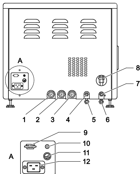
Fig. 5: Systemec DX 23; back view
