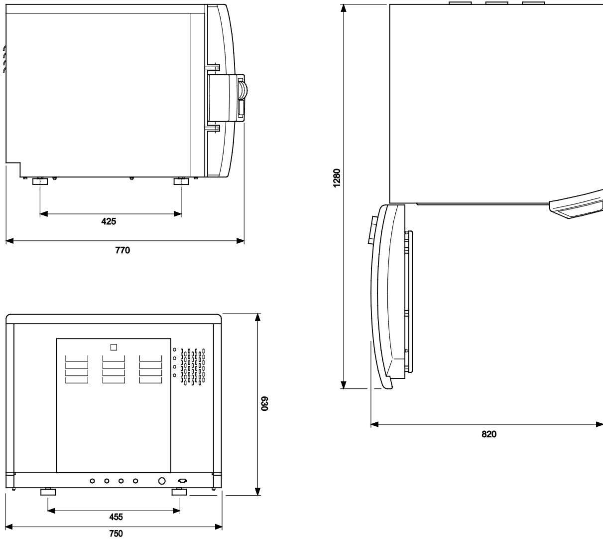
Fig. 3: Outer dimensions of Systemtec DX/DE-65
