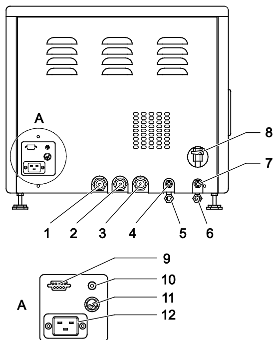
Fig. 4: Systec DX 23; back view
