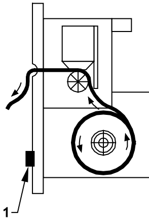
Fig. 2: Feeding the printer
