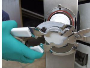
Fig. 6: Replacing filter: Removing the exhaust filter cartridge
