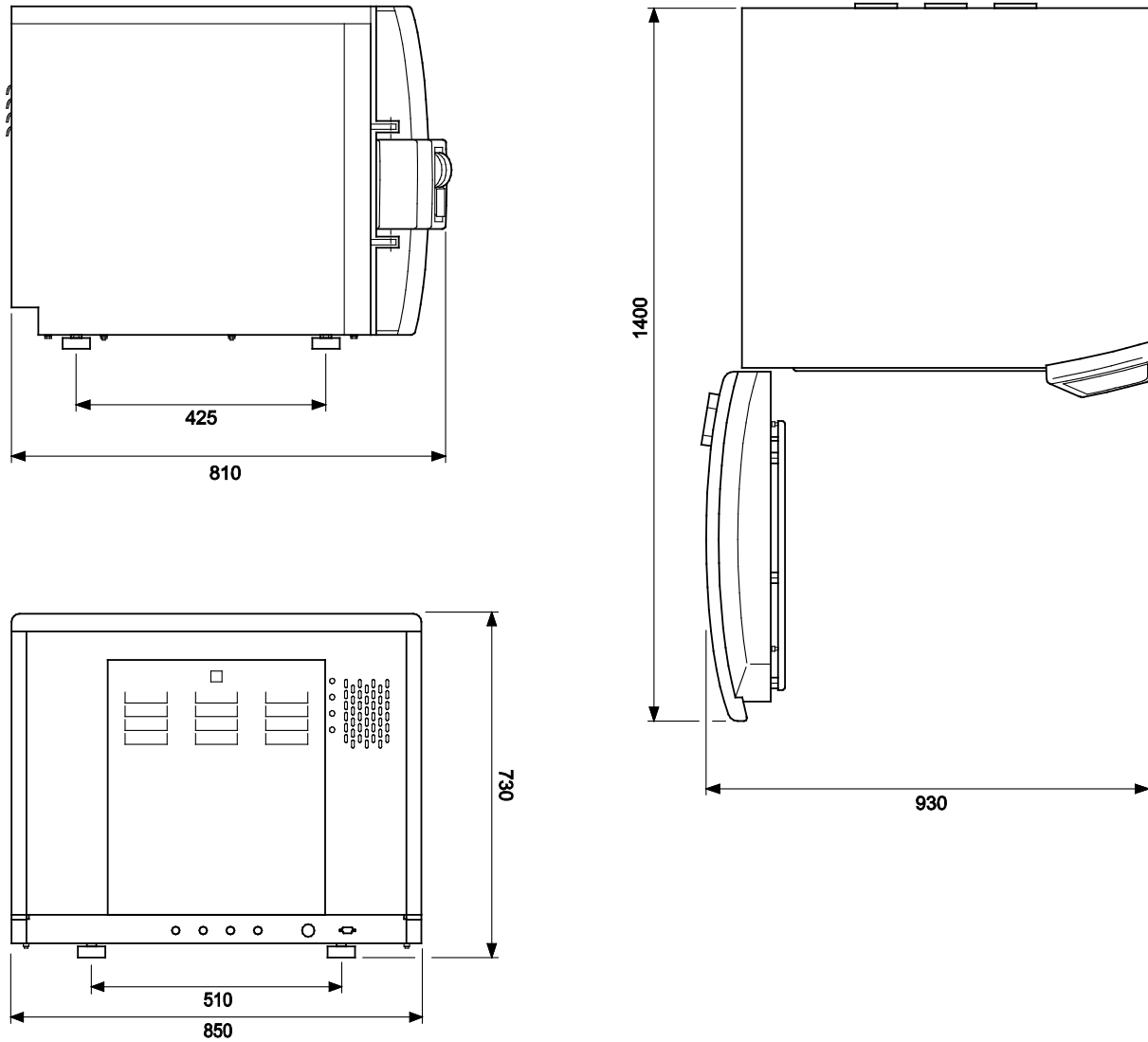
Fig. 5: Outer dimensions of Systemec DX/DE-100
